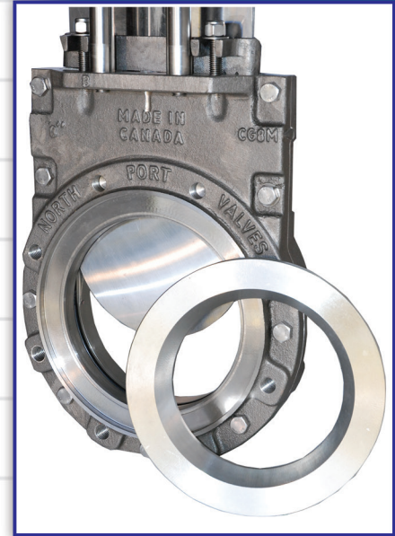
Cone Deflector before installation
